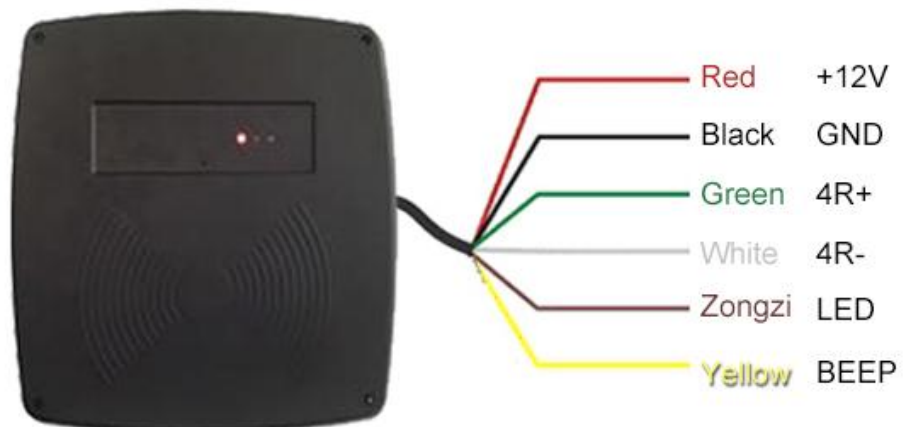
Card reader wiring diagram (485)
