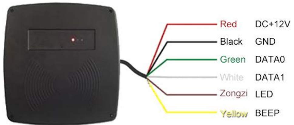
Card reader wiring diagram (Wiegand26)
